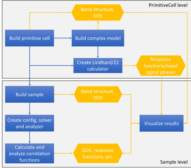
Fig. 2. Workflow of common usages of TBPLaS. Blue rectangles and orange hexagons denote the main steps and outputs, respectively. (For interpretation of the colors in the figure(s), the reader is referred to the web version of this article.)
