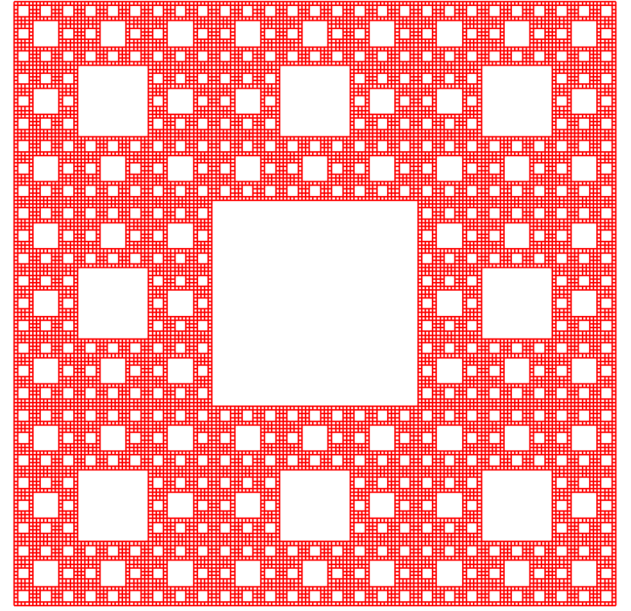
Fig. 8. Sierpiński carpet with S = 2 , L = 3 and I = 4 .
